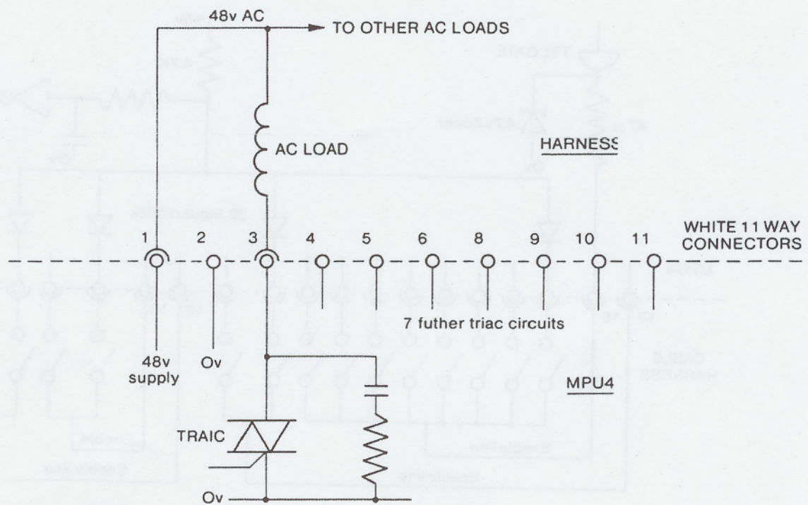
FIGURE 19 TRIAC CIRCUITS
