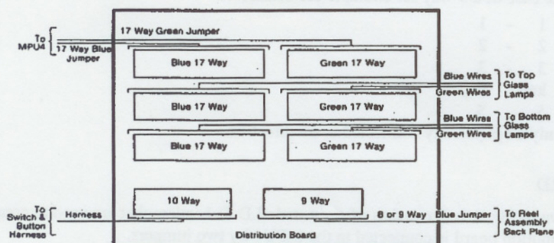
FIGURE 1.1 MAIN HARNESS DISTRIBUTION BOARD
