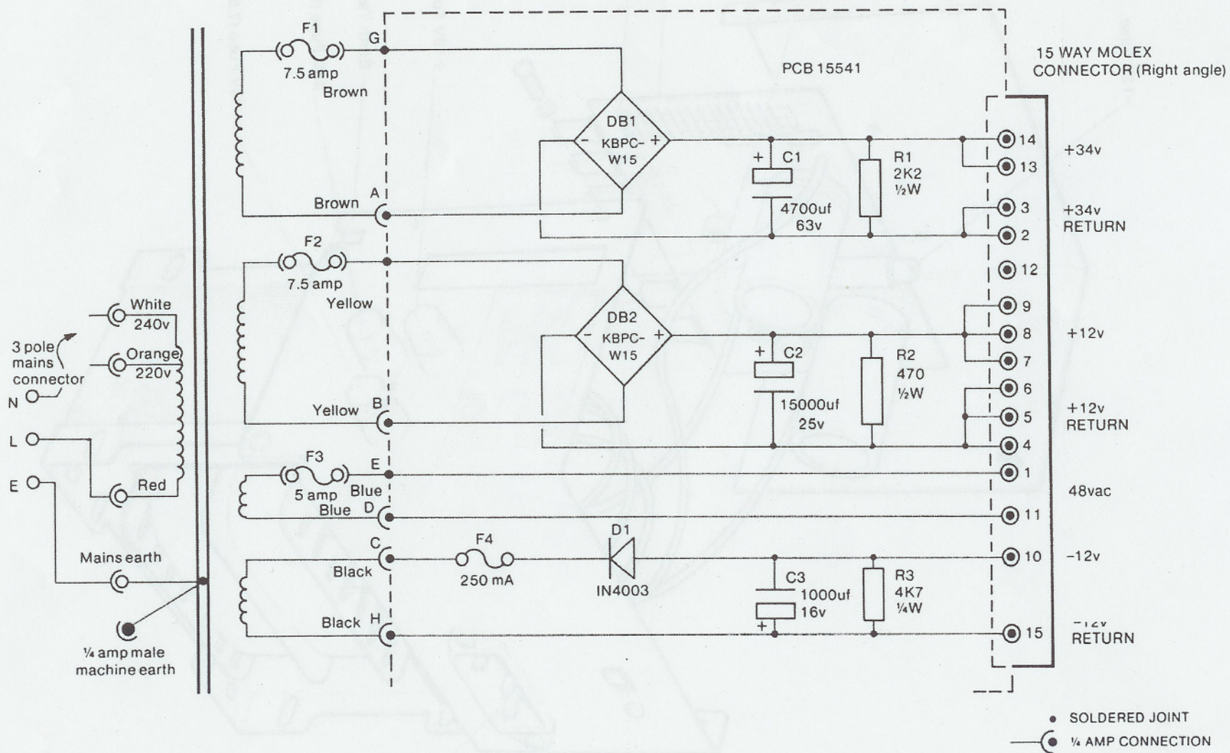
FIGURE 8 POWER SUPPLY CIRCUIT DIAGRAM
