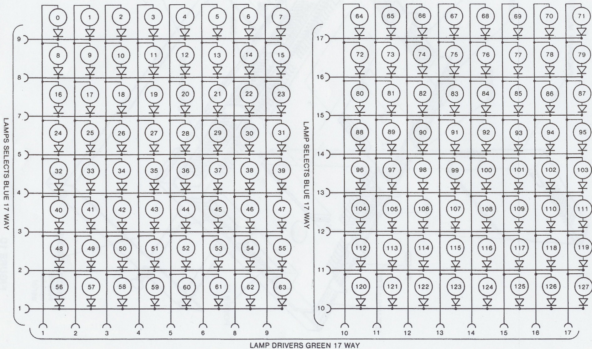
FIGURE 11 LAMP DISPLAY CIRCUIT
