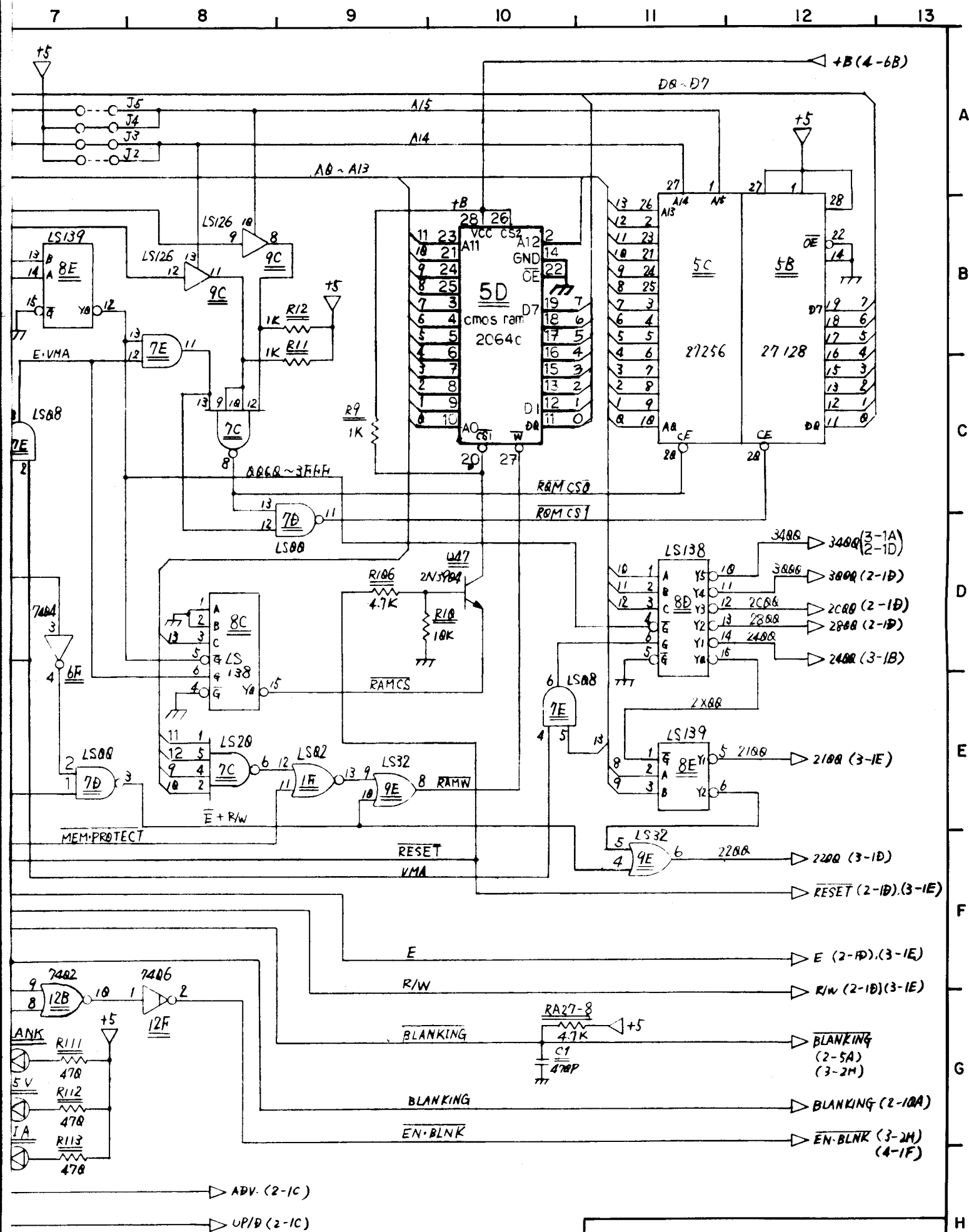
CPU BOARD 1 OF 4
